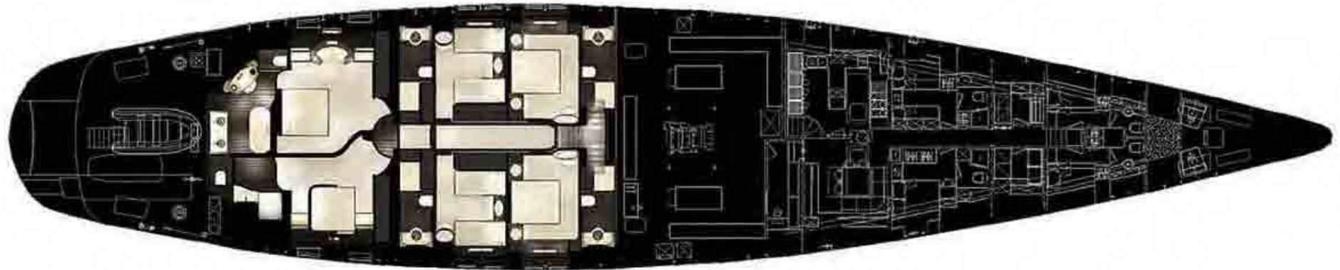
Lower Deck Layout - 6 Cabins configuration
