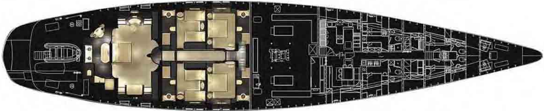
Lower Deck Layout - 5 Cabins configuration
